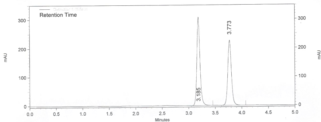
Figure 8 : Chromatogram of intermediate precision
